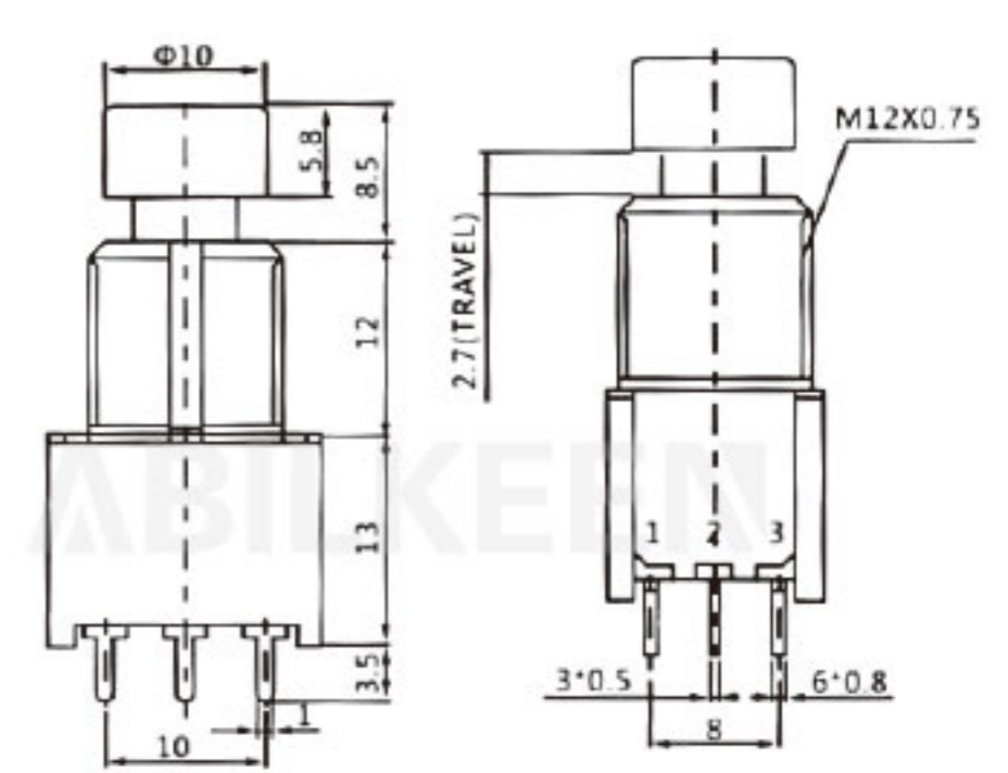
PBS-24-302SP ON-ON PBS-24-312SP ON-(ON) 2A 250VAC 4A 30VDC
