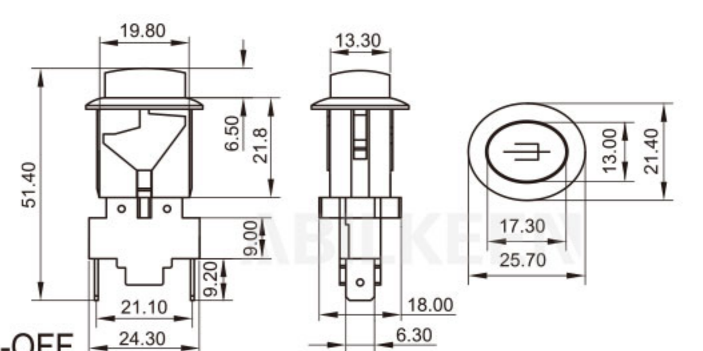
IPS-1503A ON-OFF IPS-1503B OFF-(ON)
