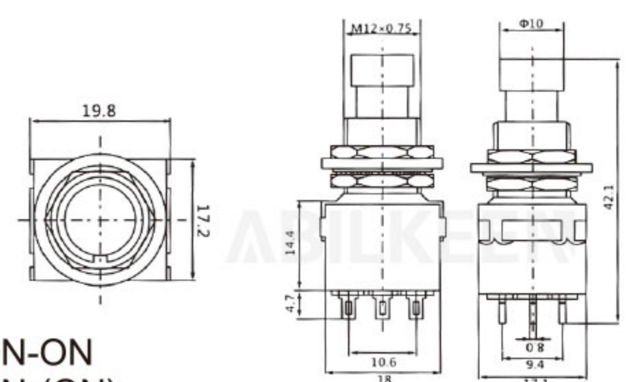
PBS-24-102 ON-ON 3P PBS-24-112 ON-(ON) 3P PBS-24-202 ON-ON 6P PBS-24-212 ON-(ON) 6P
